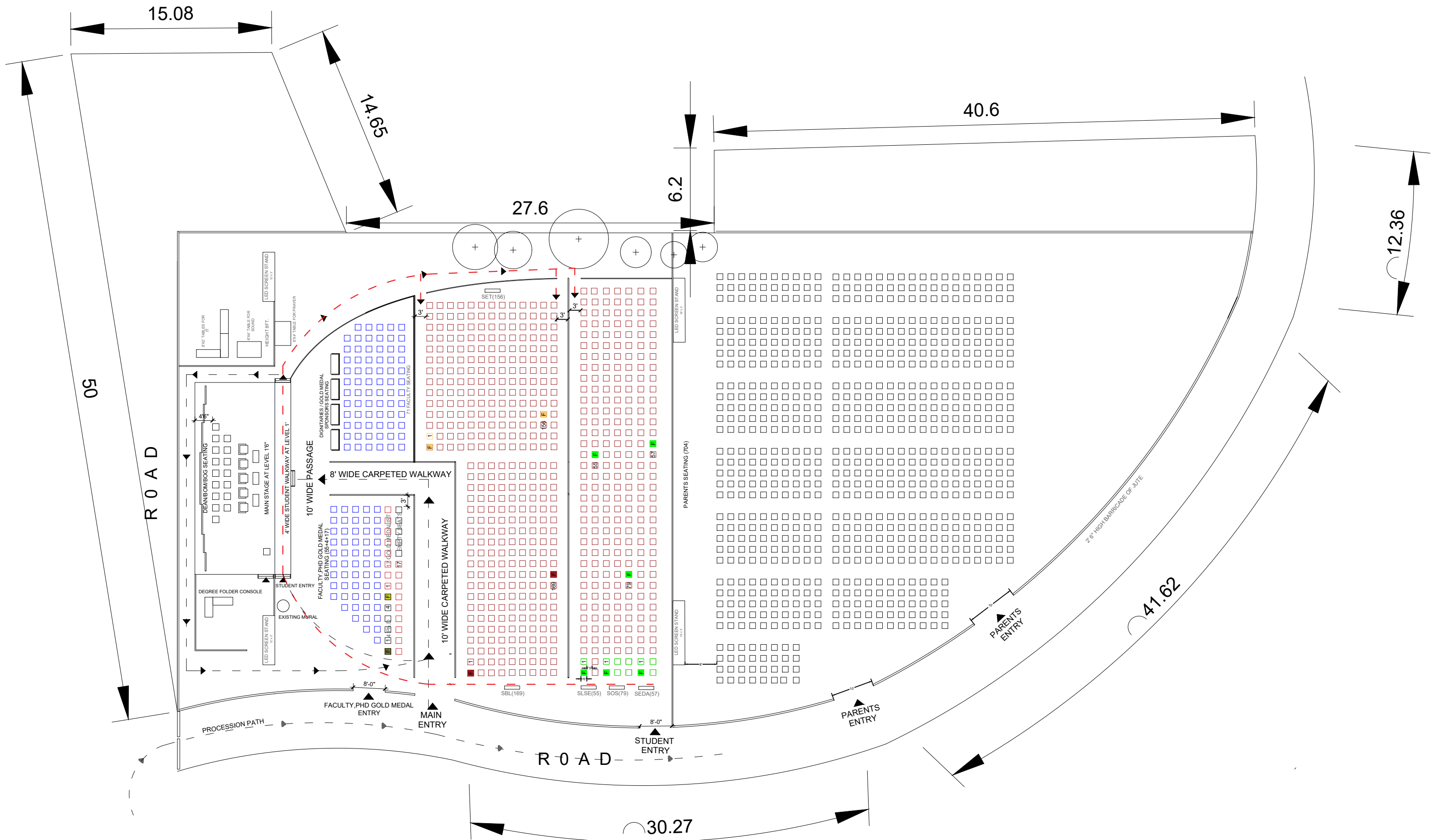
Updated Final Layout 20/11/24
